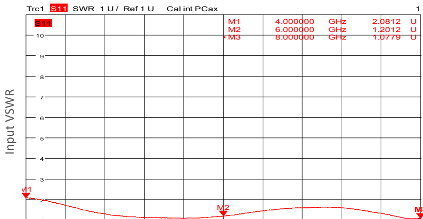
Input VSWR vs Frequency
